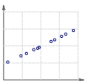
Perfect positive correlation
