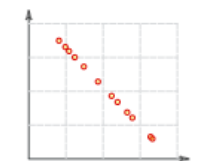
Perfect negative correlation
