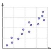
Strong positive correlation
